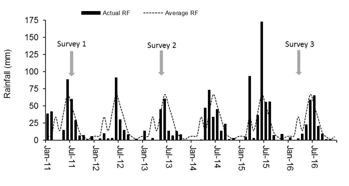
Figure 1 Mean monthly rainfall for nearby recording station at Steep Point (113.22°E, 26.18°S) and long-term average rainfall (RF=rainfall).
